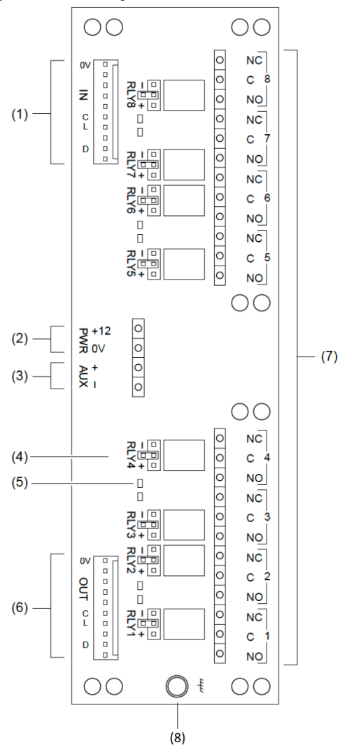
Figure 1: TS1041 layout and connectors
