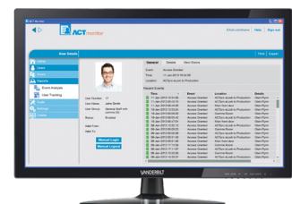
ACT Monitor
