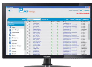
ACT Manage
