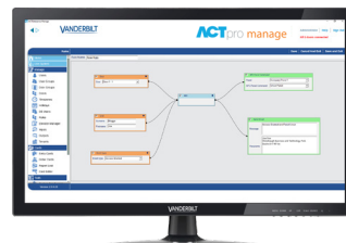
Rules Engine
