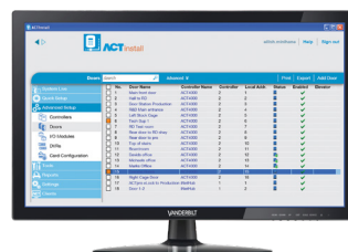
ACT Install
